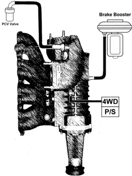
2.4 Vacuum Diagram Production Dates: 01/95-08/98
