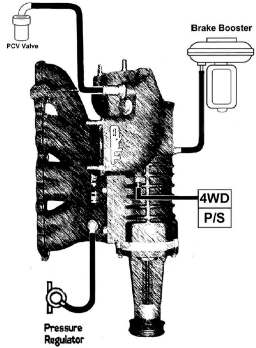
2.4 Vacuum Diagram Production Dates: 09/98 to Present
