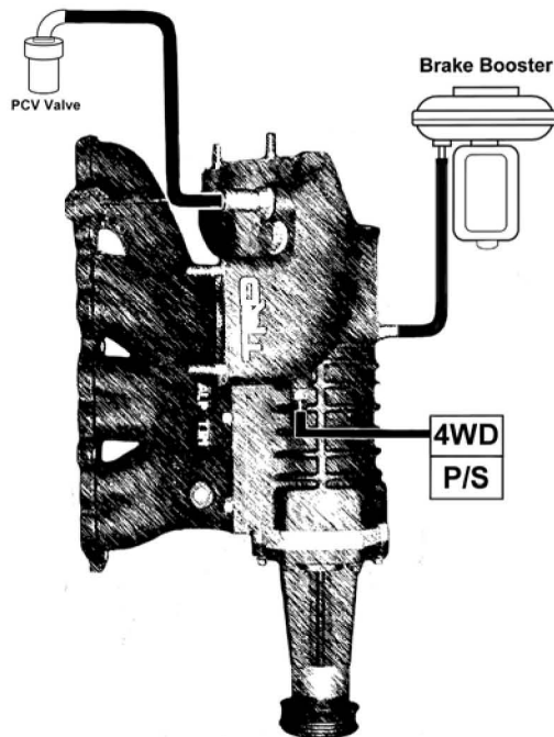
2.7 Vacuum Diagram Production Dates: 01/95 to Present
